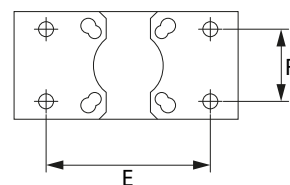
Fig. 6 (bottom view)
