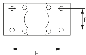
Fig. 5 (bottom view)
