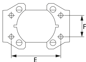
Fig. 7 (bottom view)
