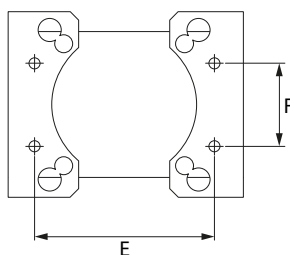
Fig. 3 (bottom view)
